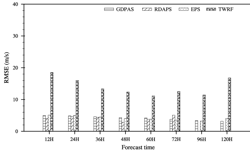
2014 Root Mean Square Error_STS
