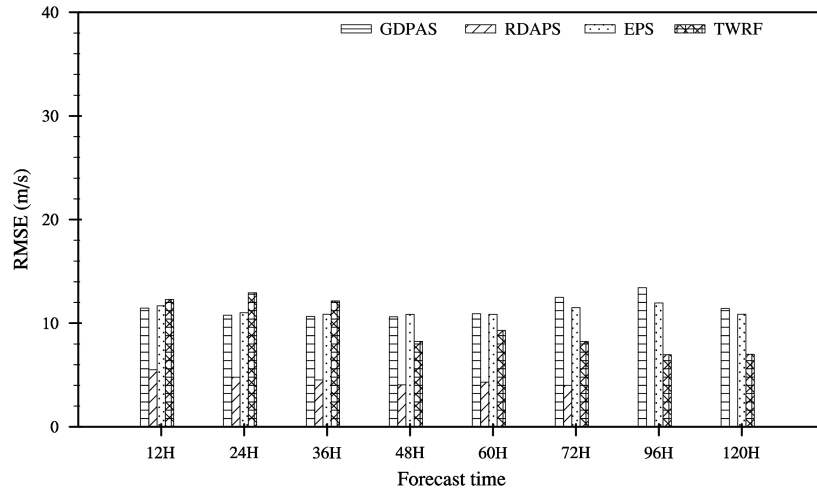
2014 Root Mean Square Error_TY
